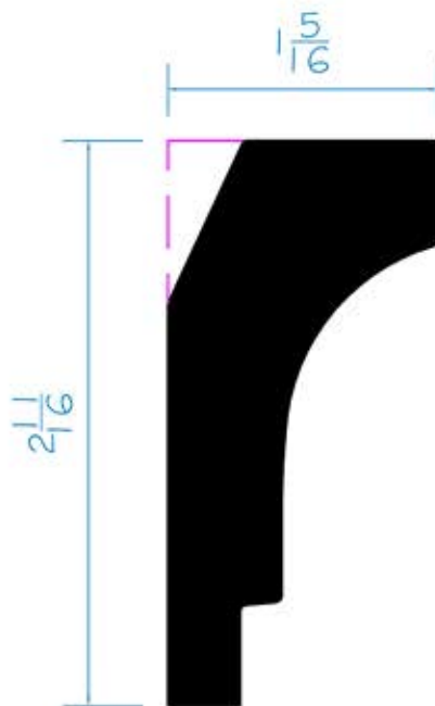
DSC-537 - 16 ft 1-5/16" x 2-11/16"
